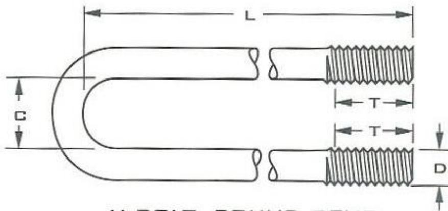
U-BOLT, ROUND BEND (D x L x C x T)
